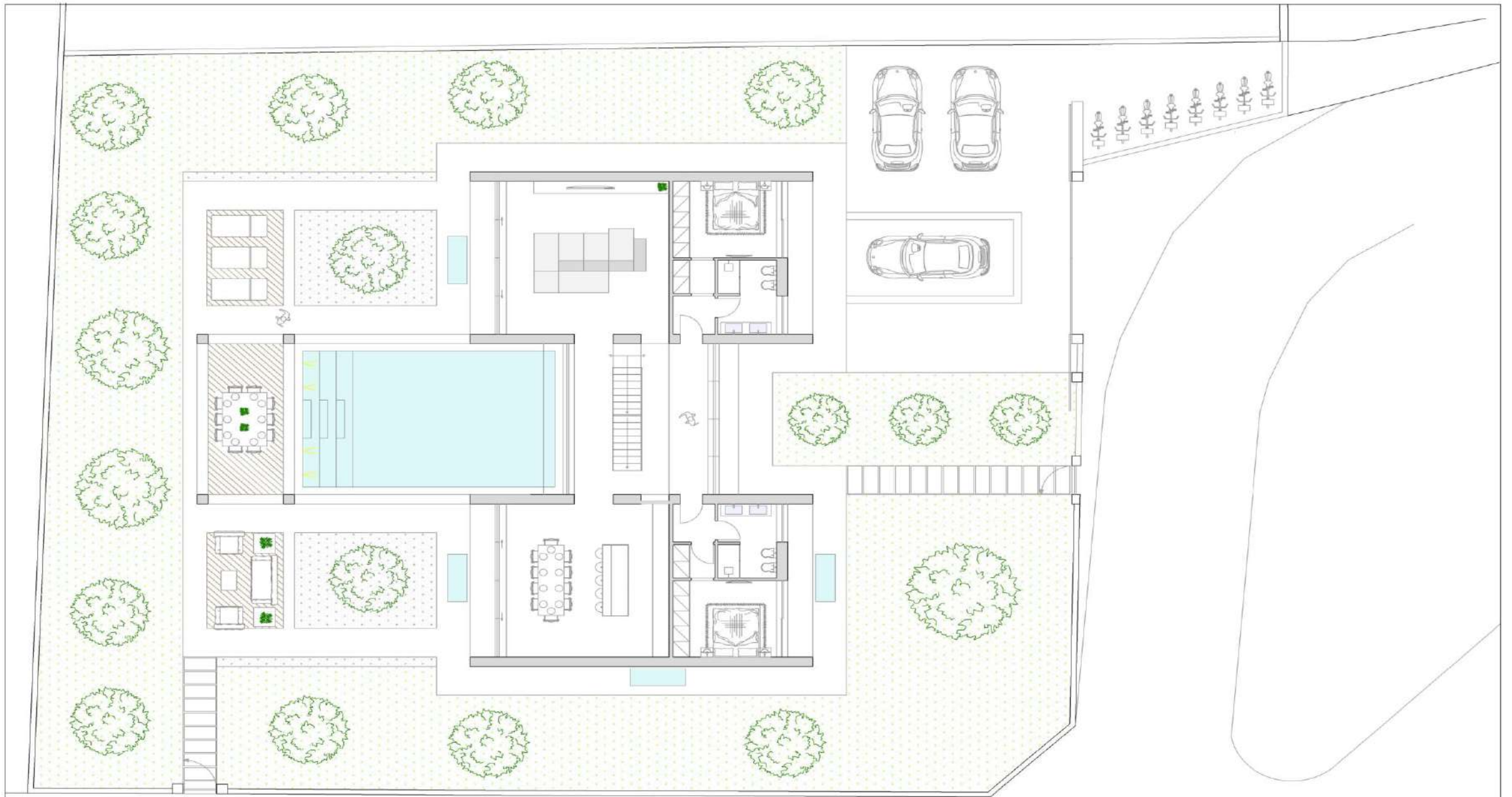
PIANO TERRA
